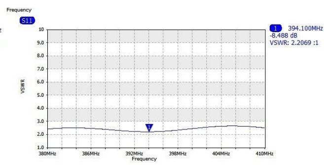
Typical SWR with matching box
