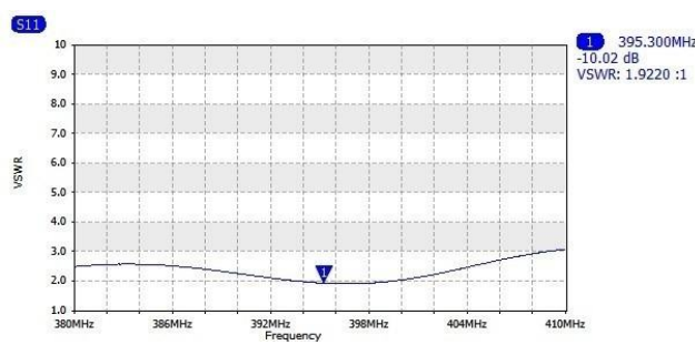
Typical SWR w/o matching box
